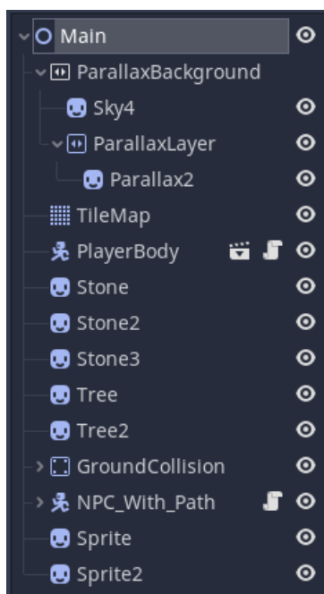
Figure 207: How a scene tree looks (specifically in Godot)
